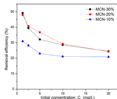
Figure 1. Removal efficiency of ^{60}\text{Co} from water of Neris River depending on initial concentration using MCN nanocomposites with different loadings (10 %, 20 %, 30 %).
