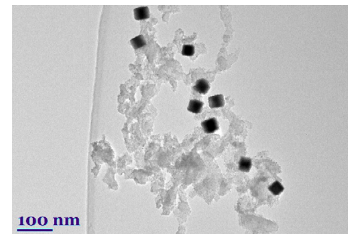
Figure 1. TEM image of Ag nanocubes loaded on the \text{CoFe}_2\text{O}_4/\text{g-C}_3\text{N}_4 .
