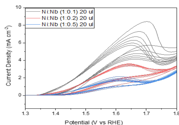
Figure 1. CV curves for methanol oxidation of \text{Ni}(\text{OH})_2 modified with \text{Nb}_2\text{O}_5
