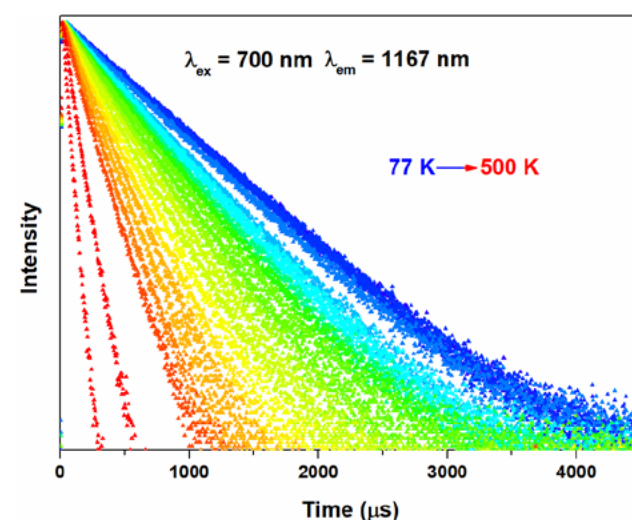
Figure 1. Temperature-dependent emission decay curves of SrClAp: \text{Mn}^{5+} .
