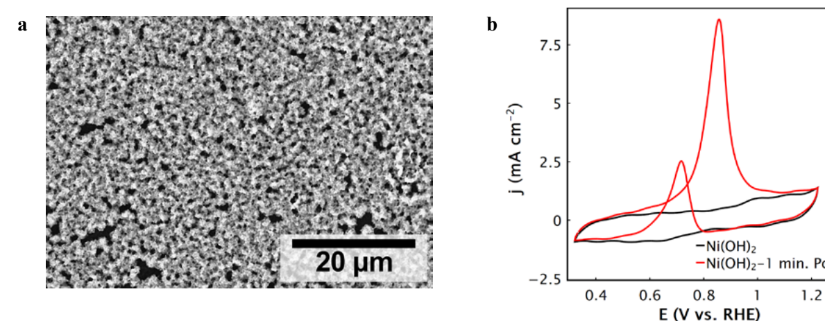
Figure 1. (a) SEM surface morphology image of a \text{Ni}/\text{Ni}(\text{OH})_2 film after 1 minute of immersion in Pd solution; (b) MOR cyclic voltammetry curves obtained in 1M KOH + 1M \text{CH}_3\text{OH} at 50 mV s -1 .
