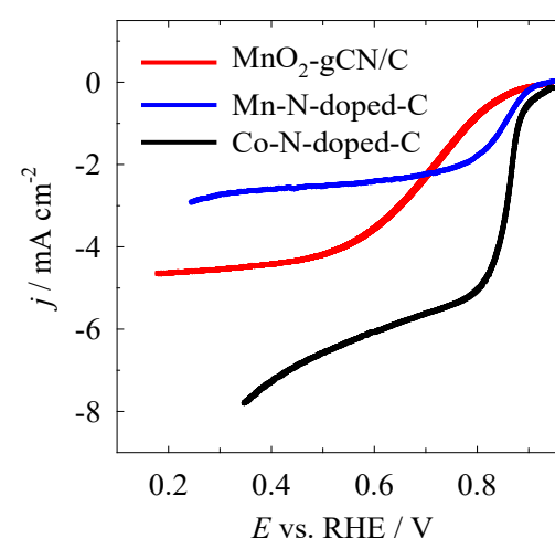
Figure 1. Comparison of Mn-N-doped-C, Co-N-doped-C, and MnO 2 -gCN-C electrocatalytic activity in O 2 -saturated 0.1 M KOH solution at 1600 rpm at 10 mVs -1
