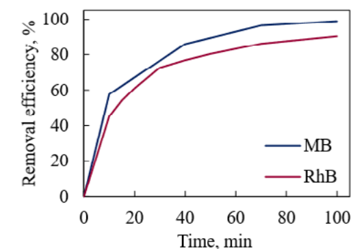
Figure 1. Efficiency of methylene blue and rhodamine B removal depending on time
