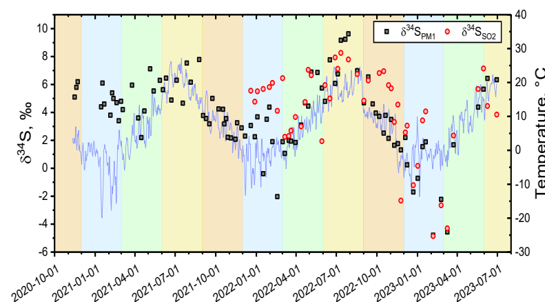
Figure 1. Seasonal variation of \delta^{34}\text{S} values of SO 2 gases ( \delta^{34}\text{S}_{\text{SO}_2} ) and PM 1 sulfate ( \delta^{34}\text{S}_{\text{PM}_1} ) recorded throughout the sampling period from November 11, 2020 to June 30, 2023.
