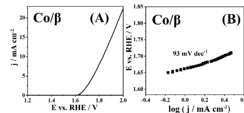
Figure 1. OER polarization curves of Co/ \beta at 20 \text{ mV s}^{-1} and 1800 rpm (A), with the corresponding Tafel plots (B).
