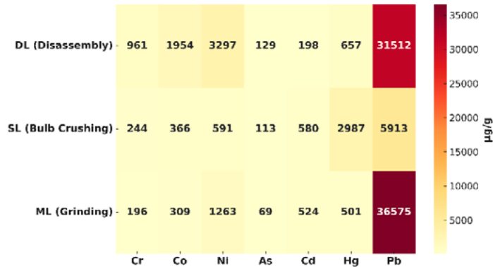
Figure 1. Concentration of selected metals (µg/g) in dust-borne particles at three e-waste recycling locations.
